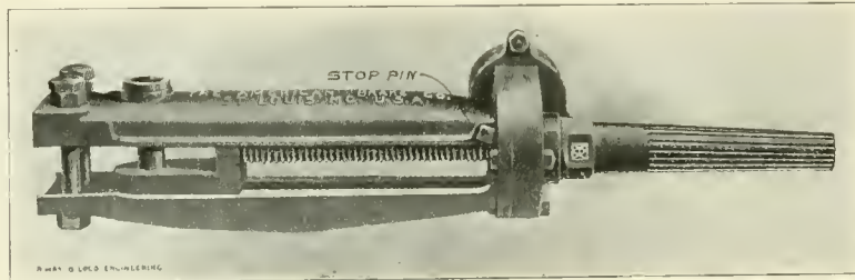
FIG. 4. STOP PIN IN ADJUSTER HOUSING
